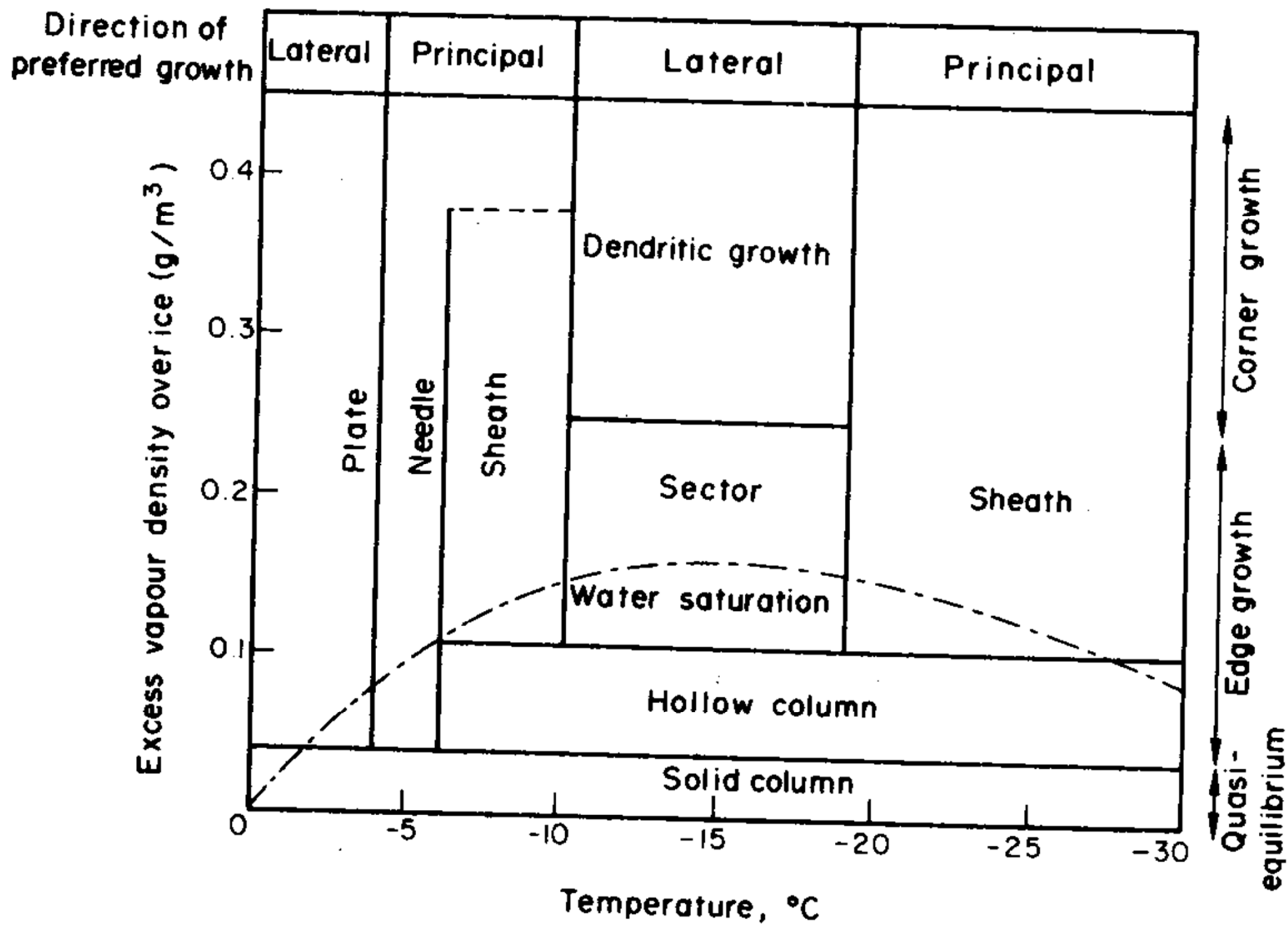
FIG 8.4 Kobayashi's diagram of ice crystal growth regimes
